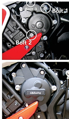
Schraube / Bolt 3 M6x35mm - 10 N/m
